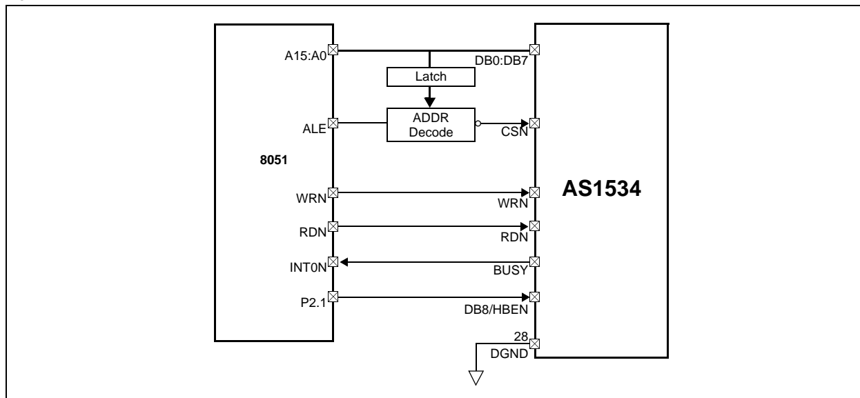
Figure 29. 8051 Interface
