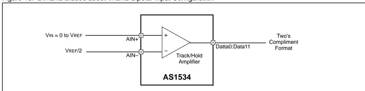
Figure 15. \pm V_{REF}/2 Biased about V_{REF}/2 Bipolar Input Configuration
