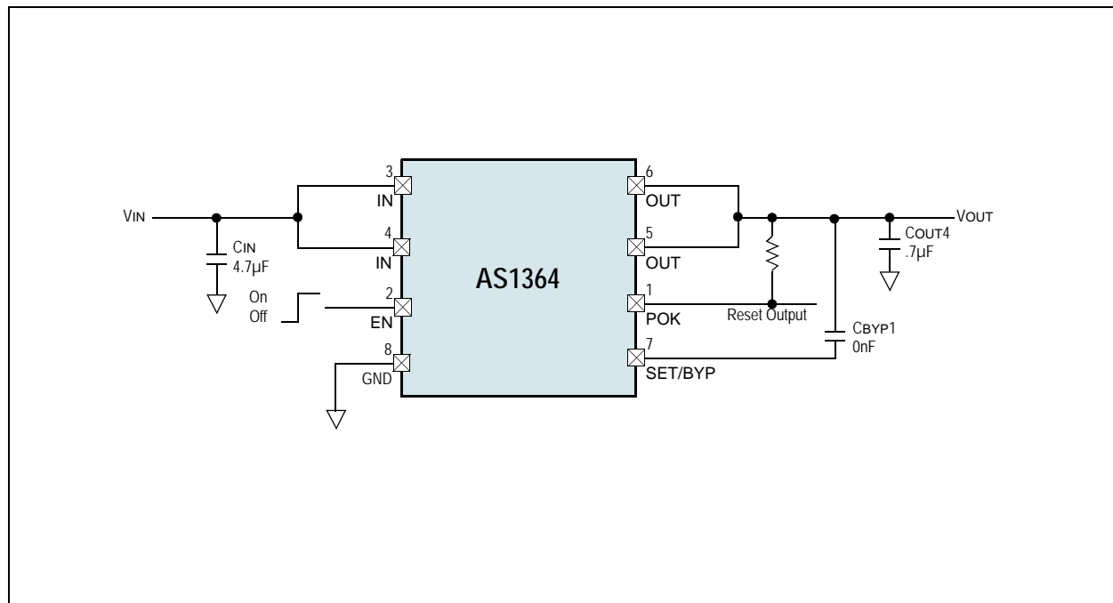
Figure 1. AS1364 - Typical Application Diagram
