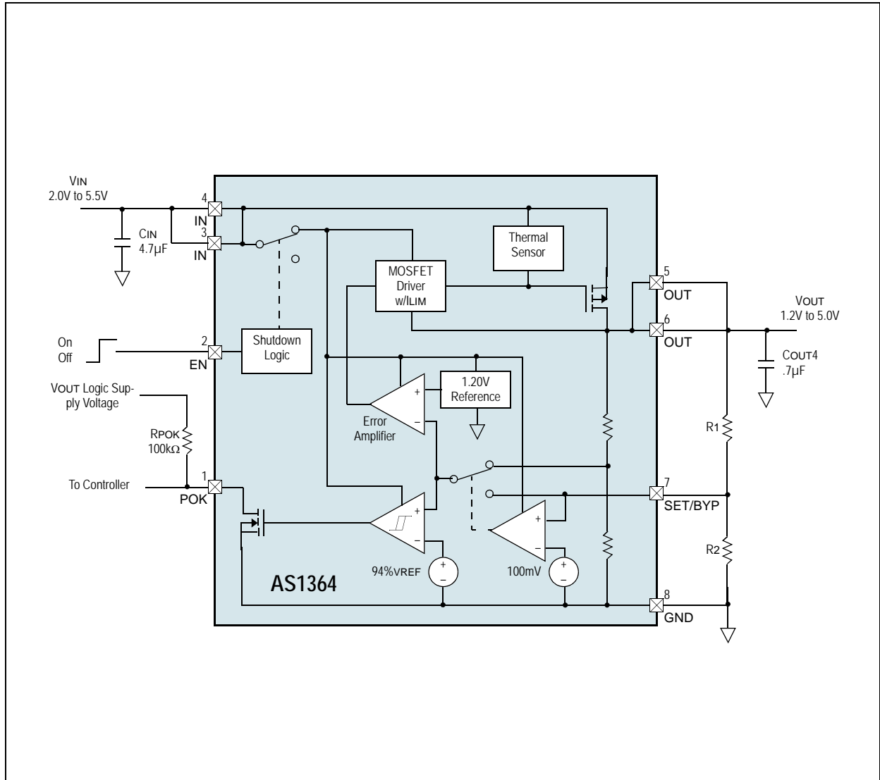
Figure 16. AS1364 - Block Diagram
