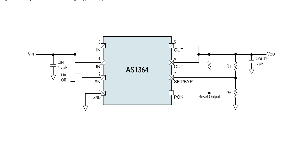
Figure 17. Adjustable Output Voltage Typical Application
