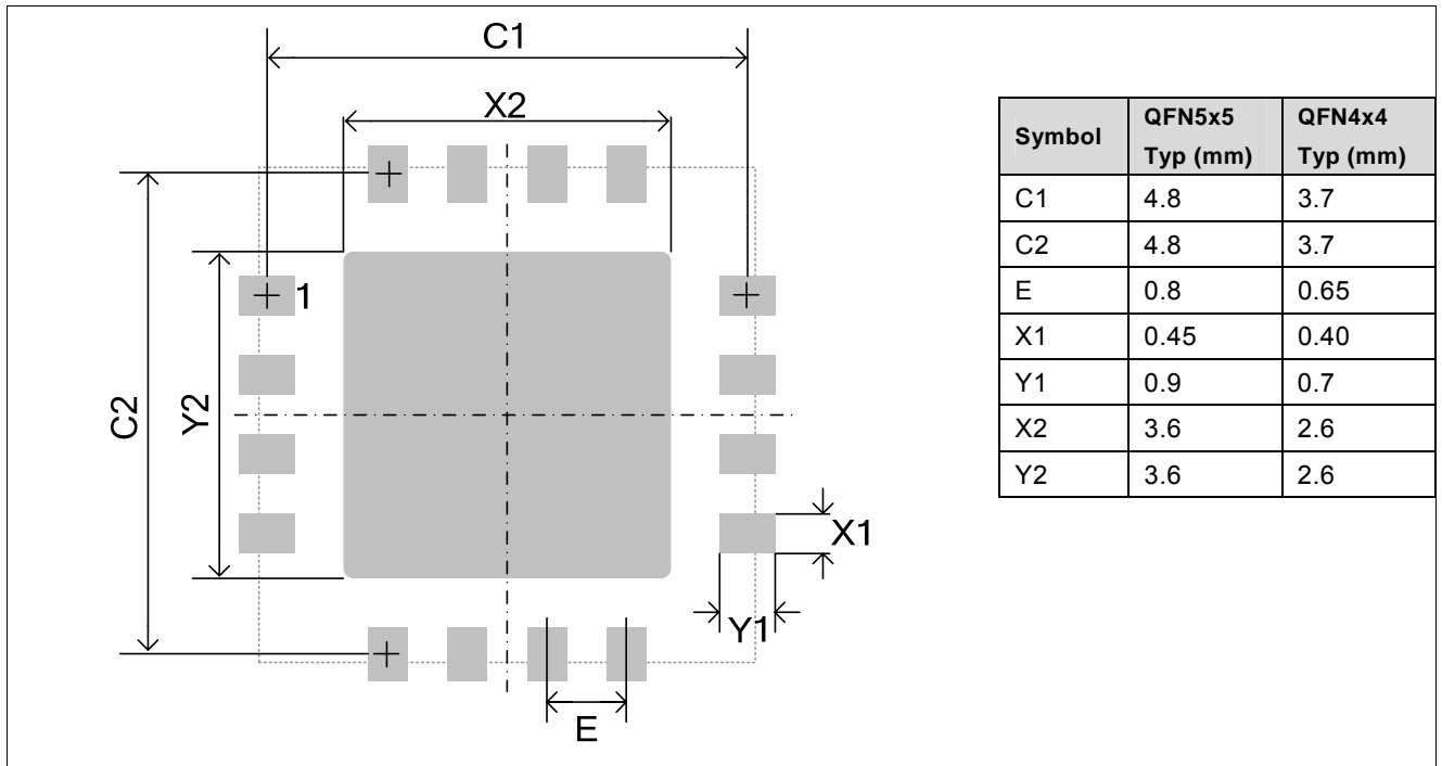
Figure 11 Recommended PCB Footprint QFN-16
