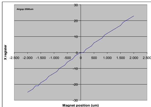
Figure 8: X Register/X Displacement (2500 \mu\text{m} Airgap)
