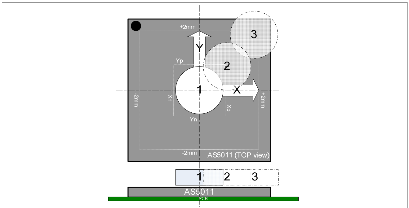
Figure 5 Position Range of the Magnet
