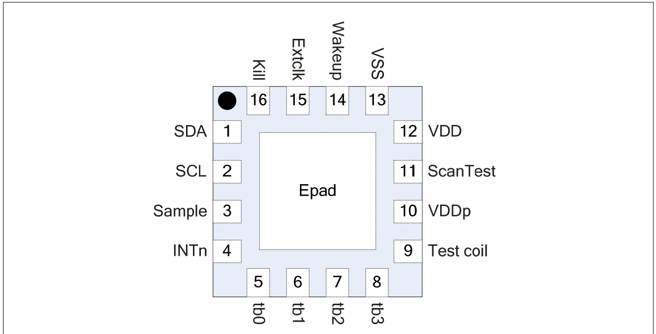
Figure 3 QFN-16 Package and Pinout (TOP view)
