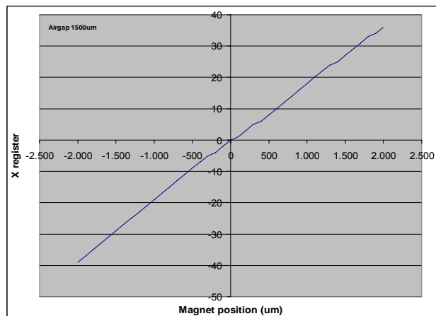
Figure 7 X Register/X Displacement (1500 \mu\text{m} Airgap)
