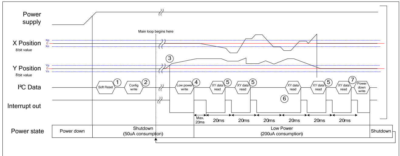
Figure 9 Typical Application Sequence for Mobile Device
