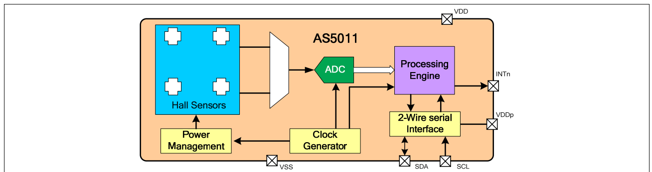
Figure 2 AS5011 Block Diagram
