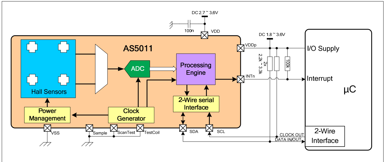
Figure 4 Electrical Connection of AS5011 with Microcontroller
