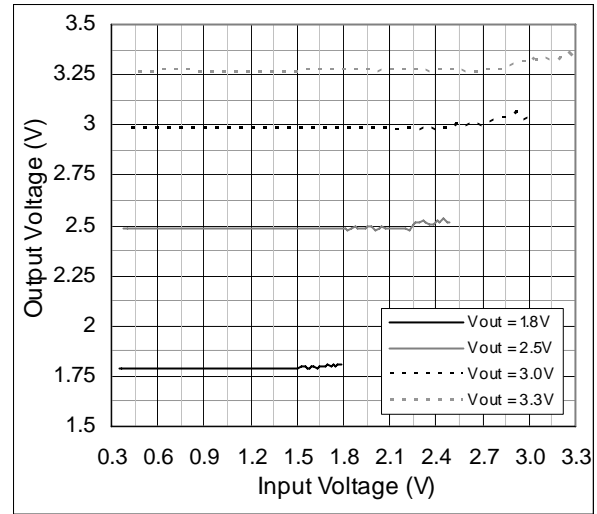
Figure 16. VOUT vs. VIN, IOUT = 10mA
