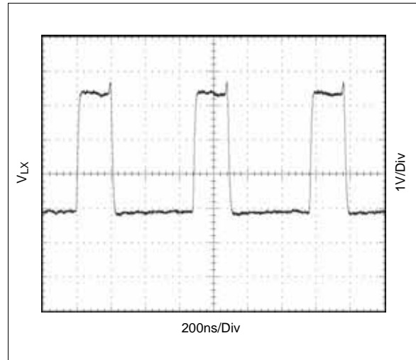
Figure 22. Coil Voltage, I_{OUT} = 100mA
