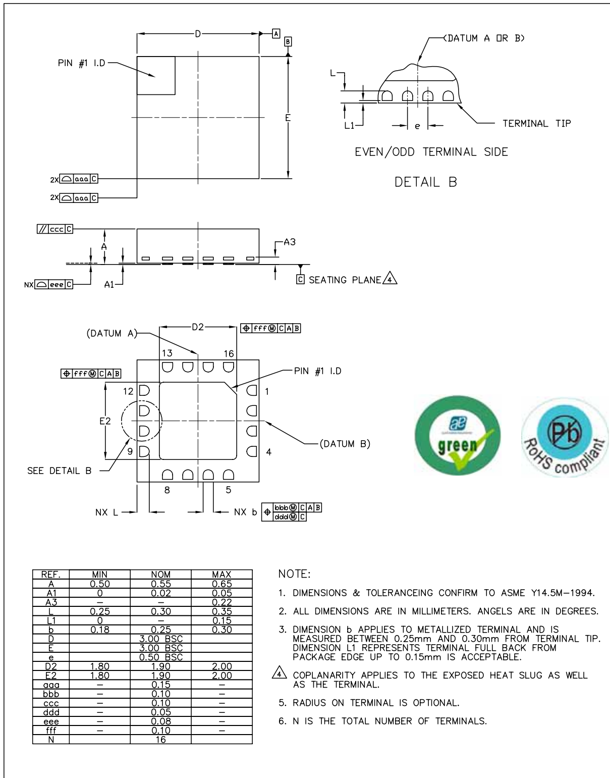
Figure 28. TQFN 3x3mm 16-pin Package
