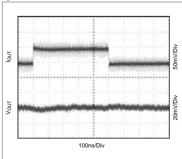
Figure 23. Load Transient
