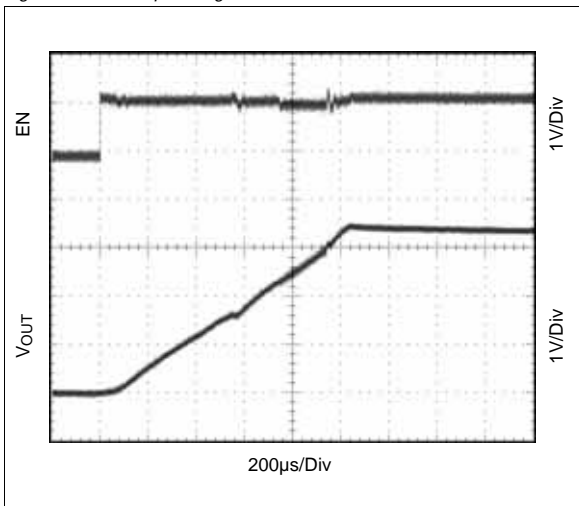
Figure 19. Startup Voltage, IOUT = 1mA
