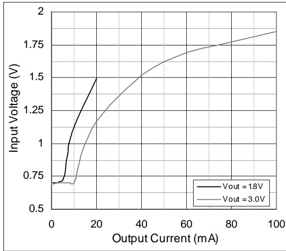
Figure 15. Startup Voltage vs. Output Current
