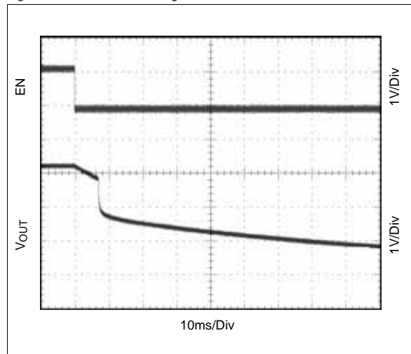
Figure 20. Shutdown Voltage, IOUT = 1mA
