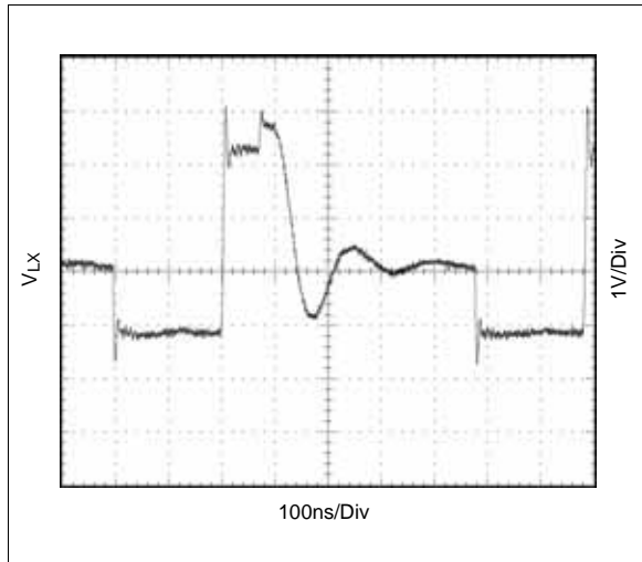
Figure 21. Coil Voltage, I_{OUT} = 1mA
